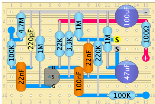
ECHOPLEX: EP-3 Preamp(Andy's)
