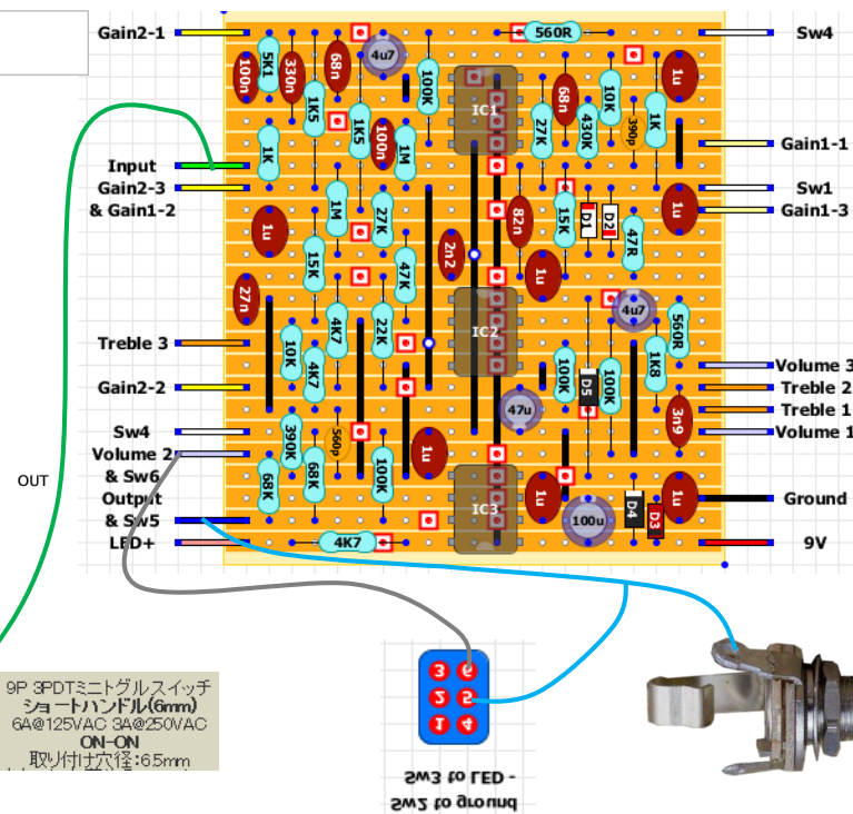
ECHOPLEX: EP-3 Preamp(Andy's)
