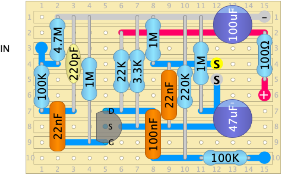
2N5484 Pinout, Pinouts
